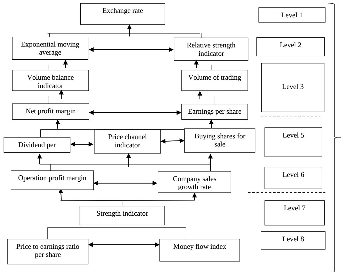
Fig. 2 Hierarchical model
