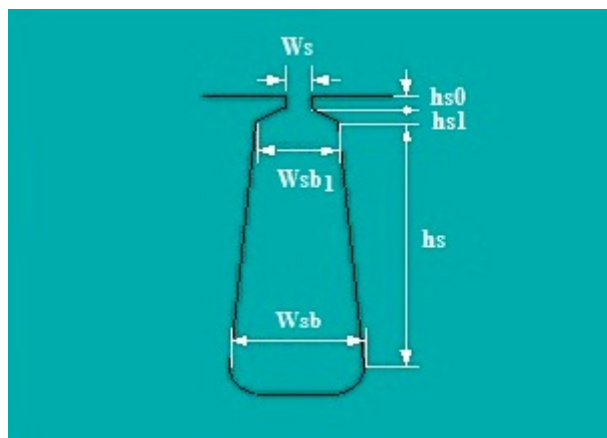
Fig. 4 Slot geometry for the radial-flux motor topology [from Maxwell13 software]
