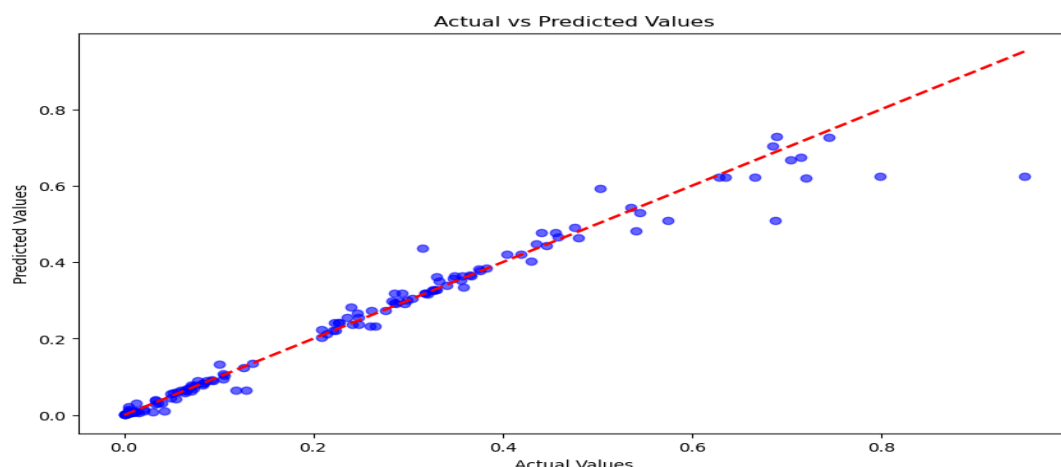
Fig. 6 Actual vs. predicted by KNN model
