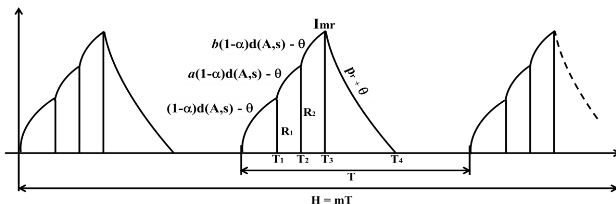
The level of inventory of imperfect products in a production-run time (0, T_1) can be formulated as:
