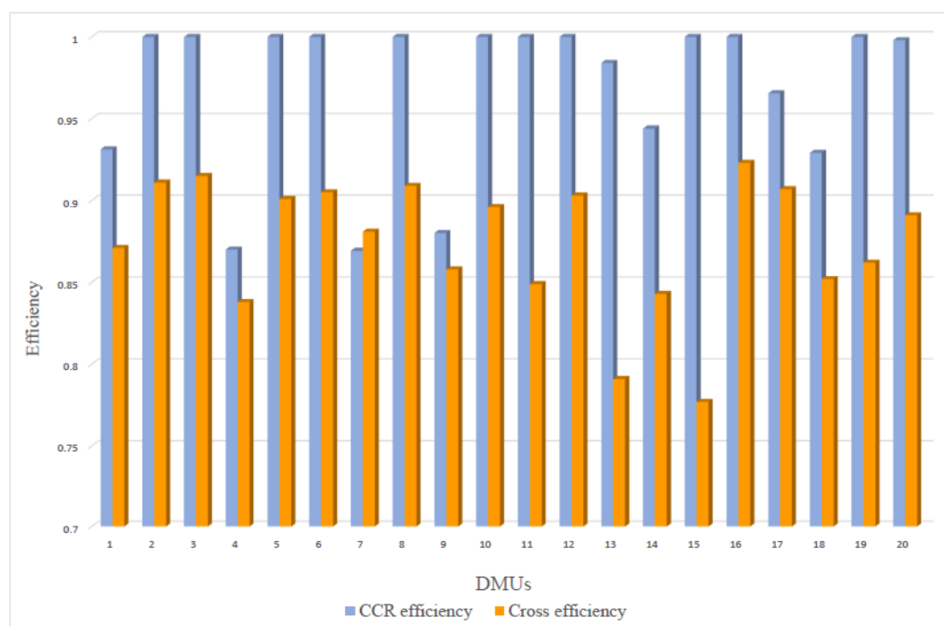
Fig. 1 Efficiency scores
