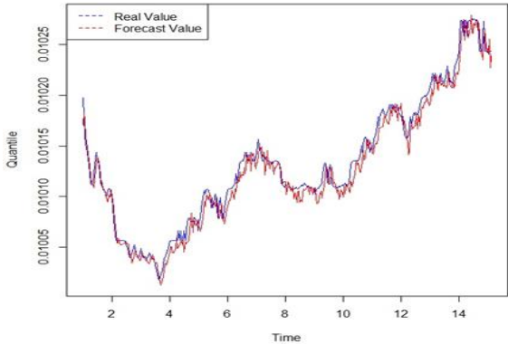
Fig. 6 Real data and forecasting value for the PCRI .
