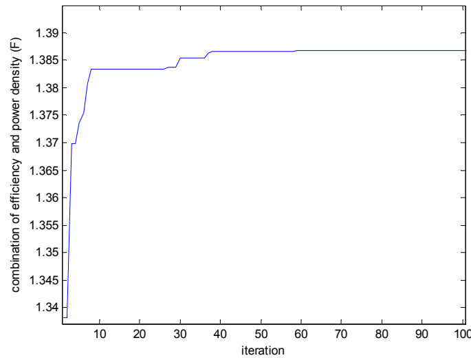
Fig 8 combination of power density and efficiency (F) versus iteration
